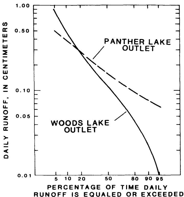
Fig. 1. Flow-duration curves for daily runoff from acidic Woods and neutral pH Panther Lakes, January 1980 through December 1981.
